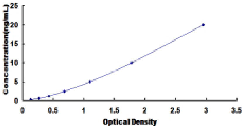
Typical Standard Curve for PDE10A ELISA.
