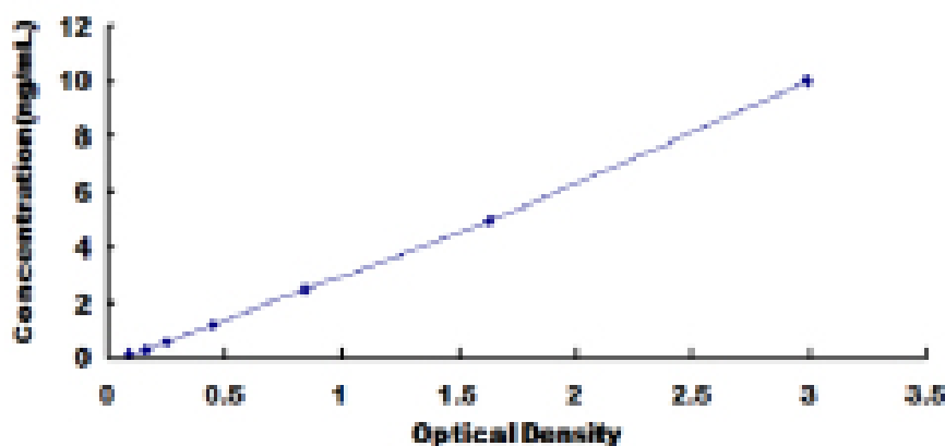
Typical Standard Curve for uPA ELISA.
