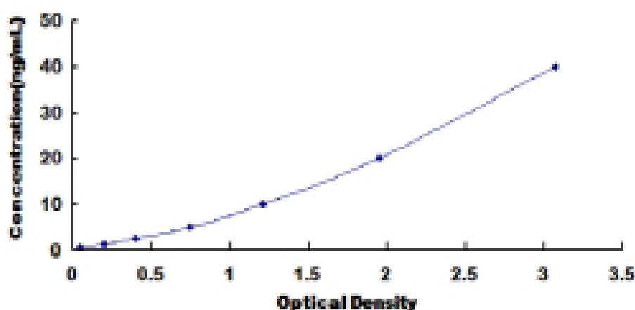
Typical Standard Curve for PKR1 ELISA.
