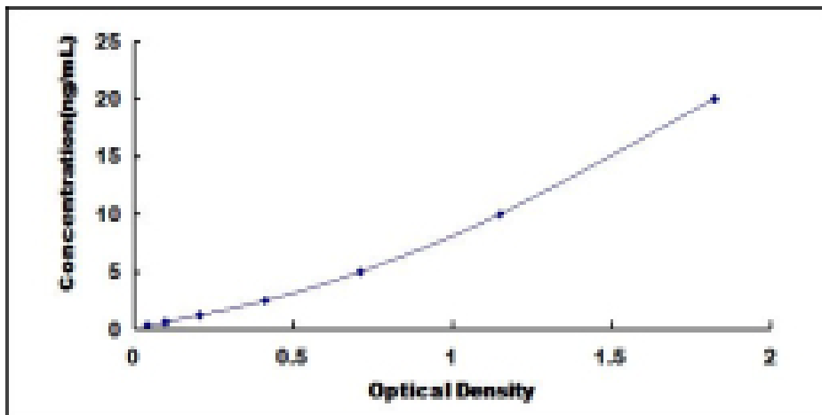
Typical Standard Curve for PRELP ELISA.
