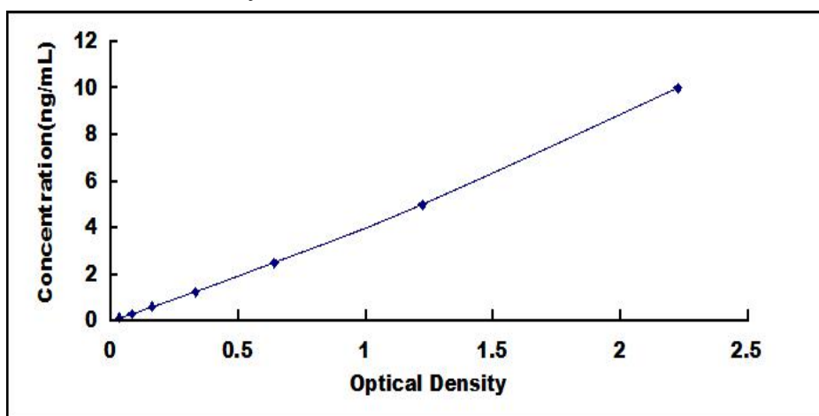
Typical Standard Curve for PSME3 ELISA.
