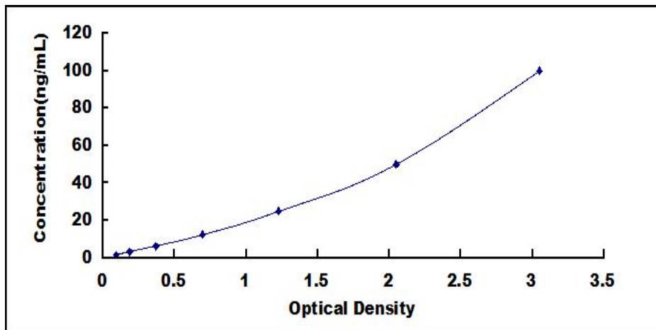
Typical Standard Curve for PKBg ELISA.
