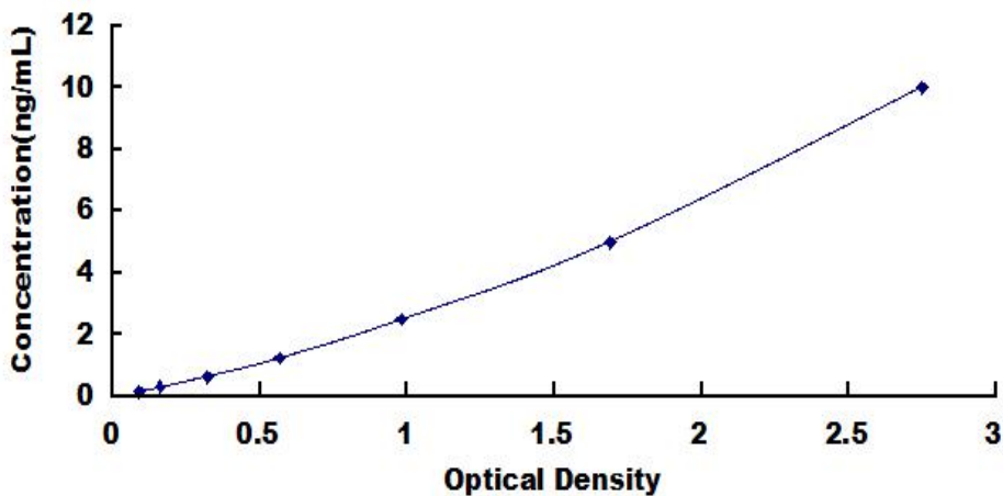
Typical Standard Curve for PTMa ELISA.
