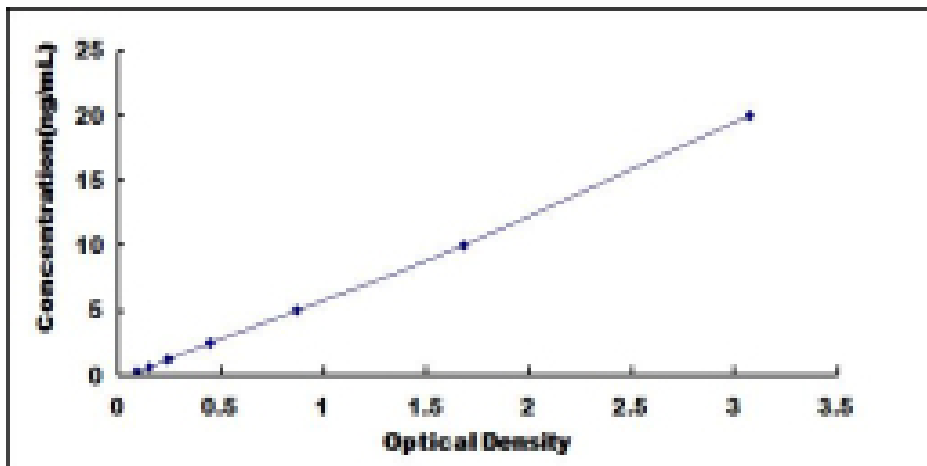
Typical Standard Curve for RIOK1 ELISA.
