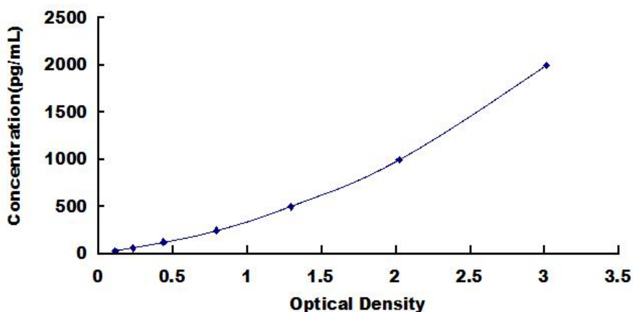
Typical Standard Curve for S100B ELISA.
