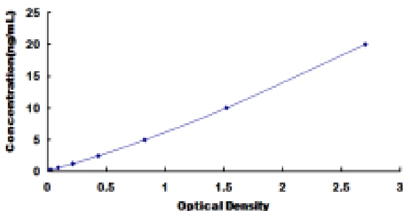
Typical Standard Curve for STH ELISA.
