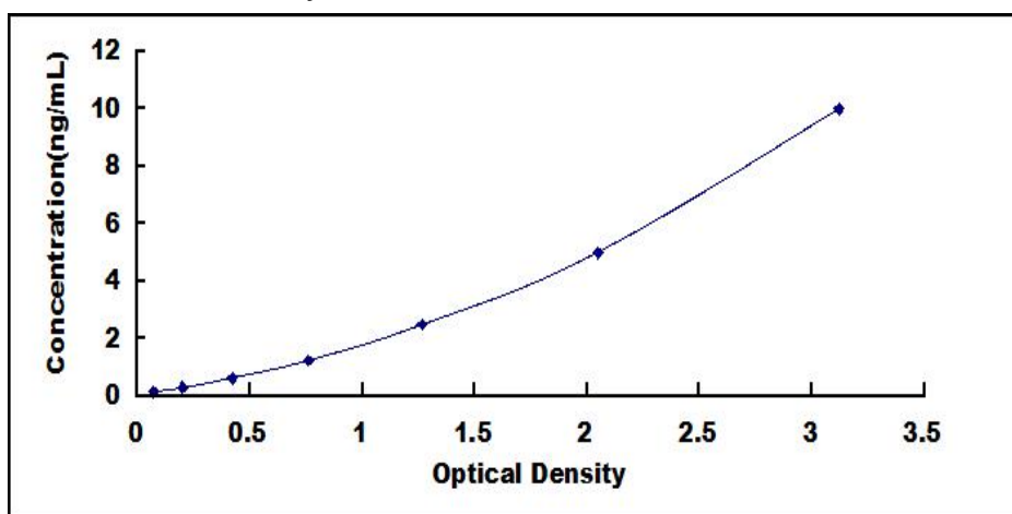
Typical Standard Curve for STAT2 ELISA.
