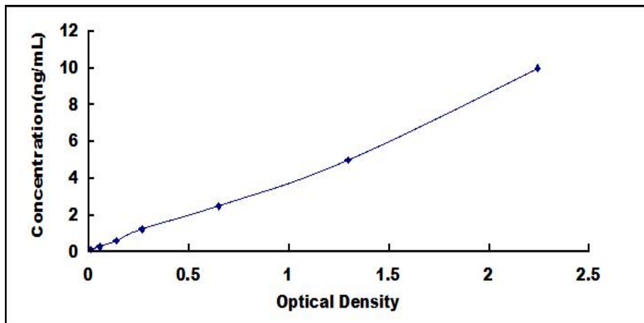
Typical Standard Curve for SNAI1 ELISA.
