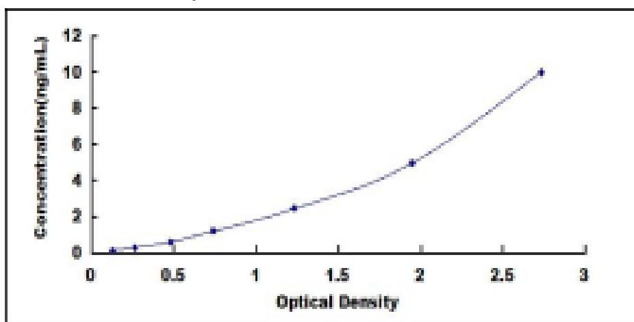
Typical Standard Curve for NIS ELISA.
