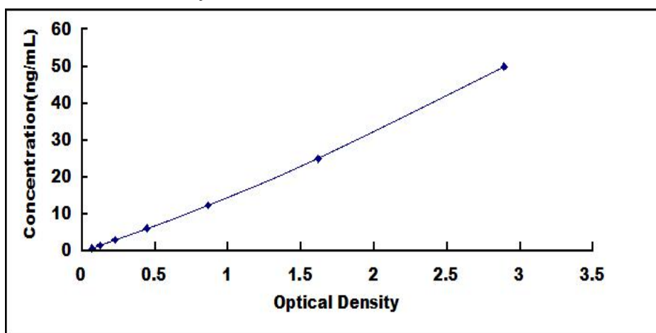
Typical Standard Curve for SOD3 ELISA.
