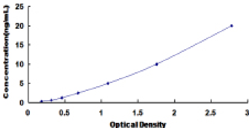
Typical Standard Curve for SYNrg ELISA.
