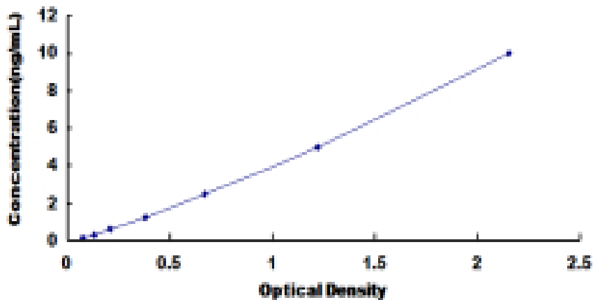
Typical Standard Curve for TOP3 ELISA.
