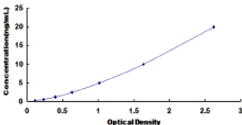
Typical Standard Curve for TSC22 ELISA.
