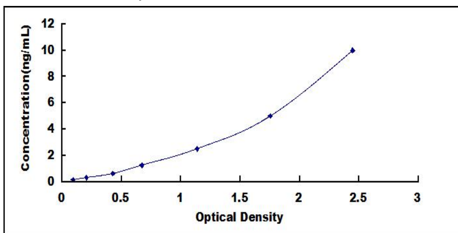
Typical Standard Curve for TAGLN ELISA.
