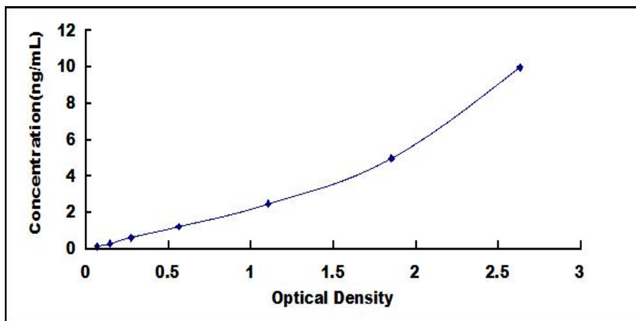
Typical Standard Curve for TFF1 ELISA.
