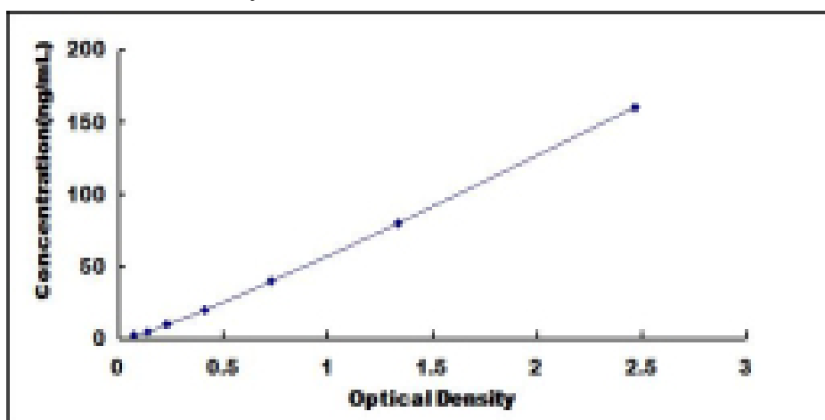
Typical Standard Curve for TNNI1 ELISA.
