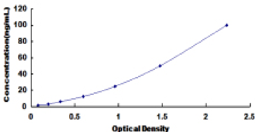
Typical Standard Curve for VEGFR2 ELISA.
