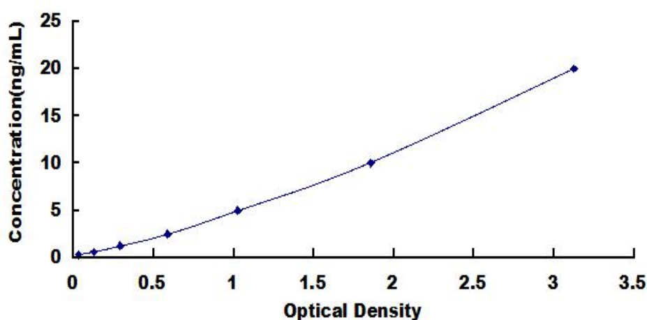
Typical Standard Curve for VGLUT1 ELISA.
