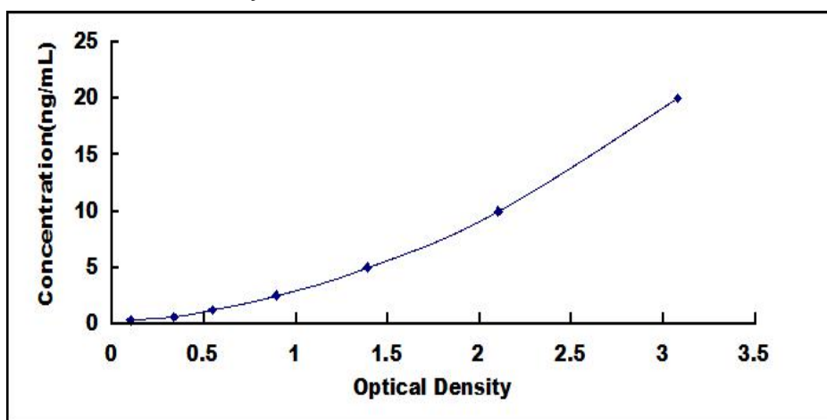
Typical Standard Curve for VIM ELISA.
