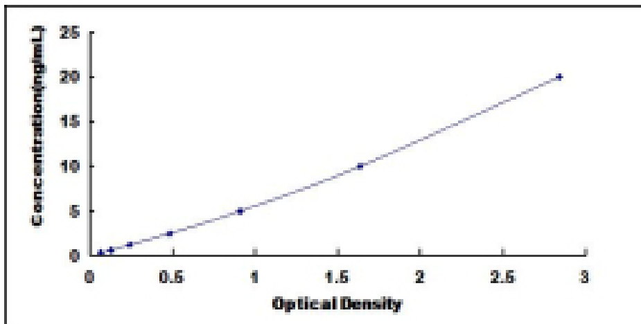
Typical Standard Curve for ZNRD1 ELISA.
