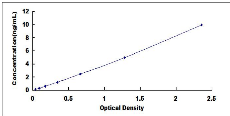
Typical Standard Curve for PAFR ELISA.
