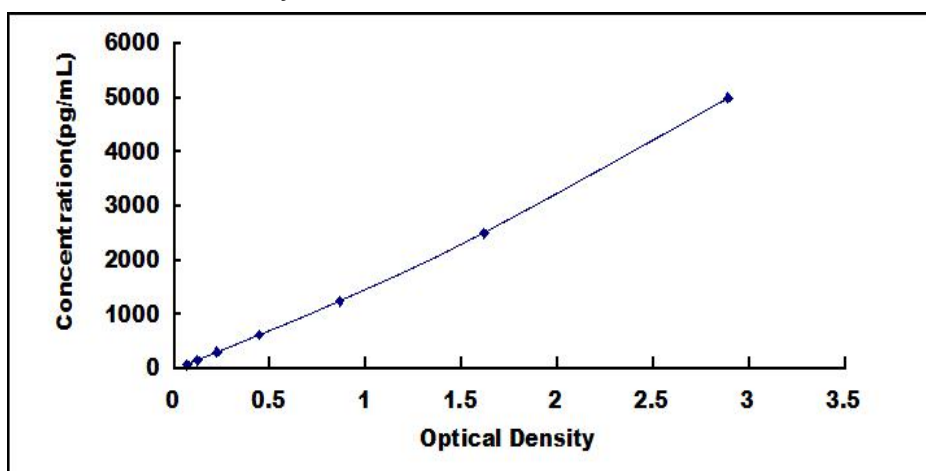
Typical Standard Curve for DPP7 ELISA.
