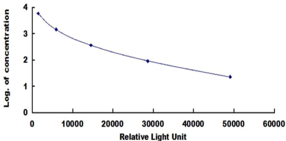
Typical Standard Curve for E1 ELISA.
