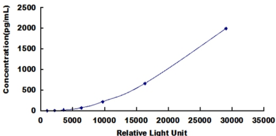
Typical Standard Curve for IL18 ELISA.
