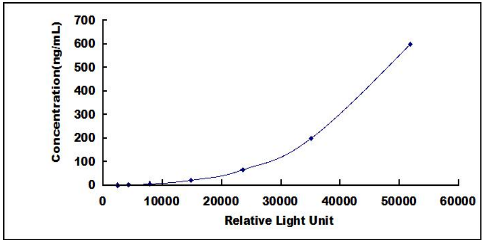
Typical Standard Curve for APOE ELISA.
