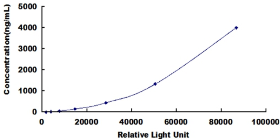
Typical Standard Curve for AT ELISA.
