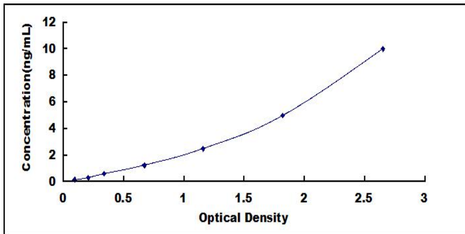
Typical Standard Curve for TrkB ELISA.
