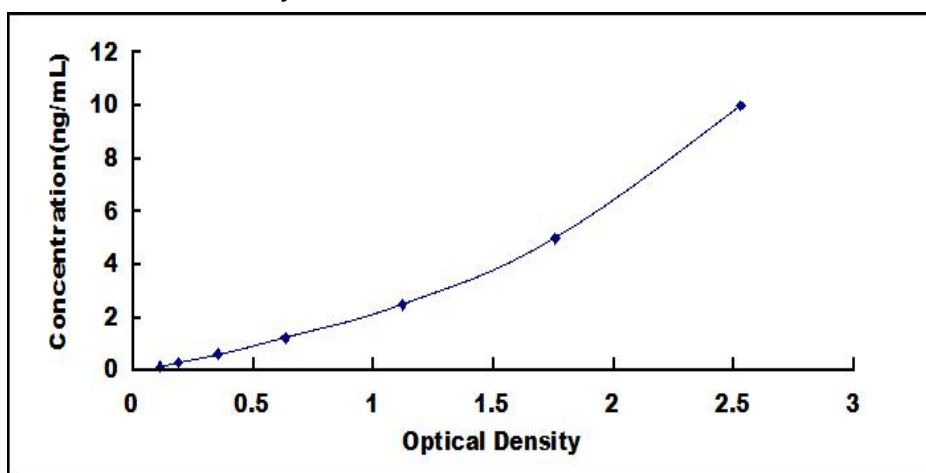
Typical Standard Curve for STMN1 ELISA.
