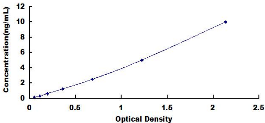
Typical Standard Curve for RHOA ELISA.
