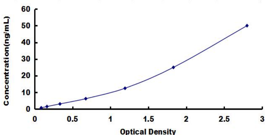
Typical Standard Curve for PI4Ka ELISA.
