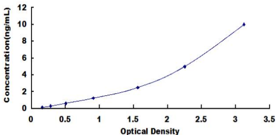
Typical Standard Curve for ETS1 ELISA.
