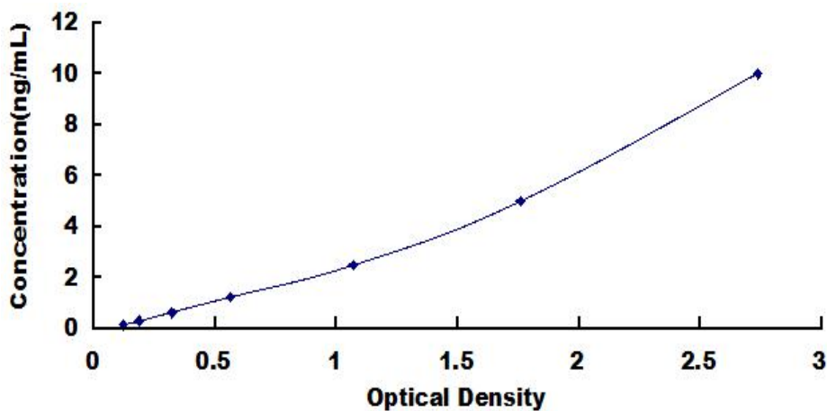
Typical Standard Curve for Sp1 ELISA.
