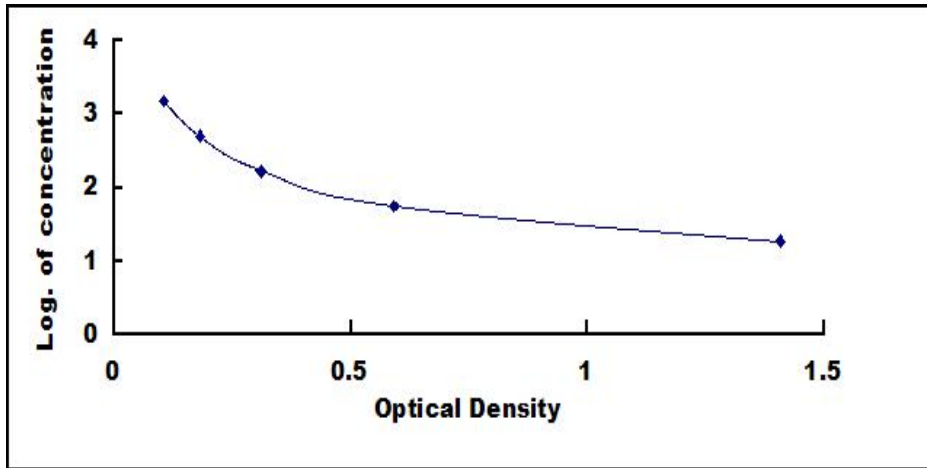
Typical Standard Curve for ADP ELISA.
