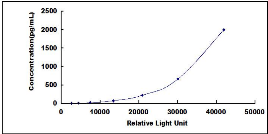
Typical Standard Curve for cTnI ELISA.
