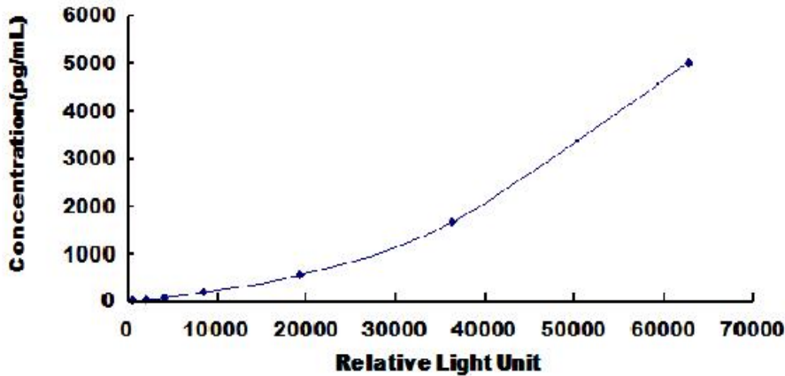
Typical Standard Curve for BNP ELISA.
