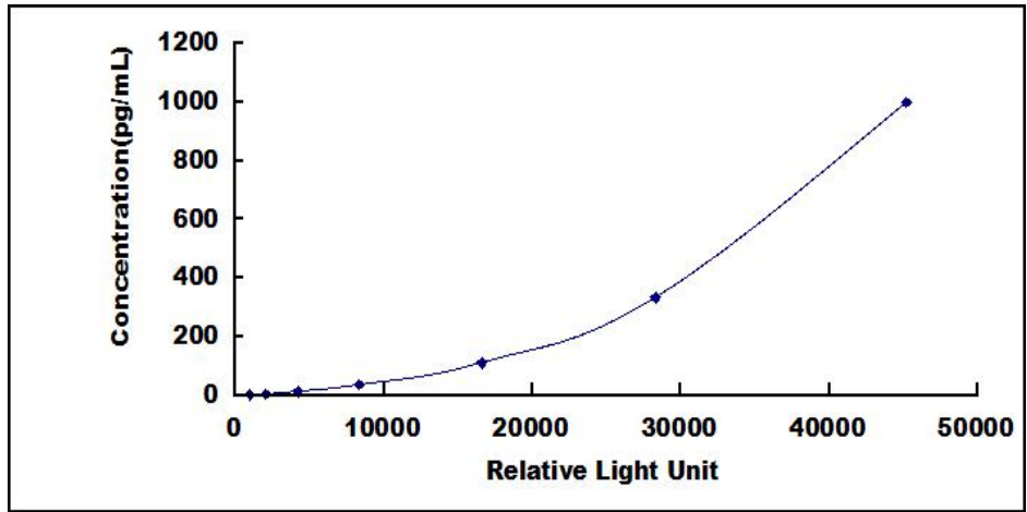
Typical Standard Curve for FGF18 ELISA.
