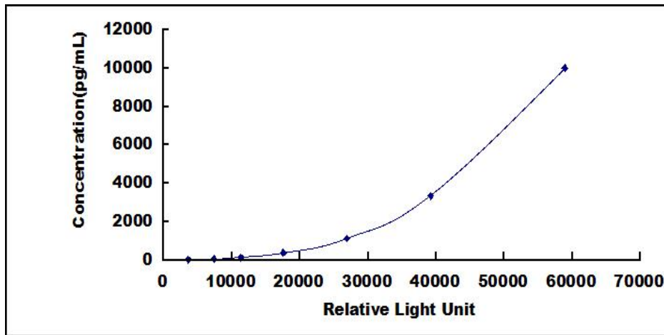
Typical Standard Curve for UBE2L3 ELISA.
