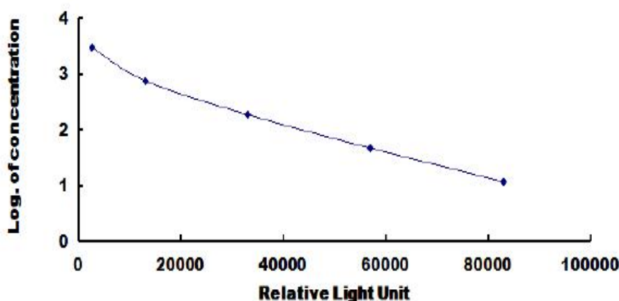
Typical Standard Curve for AngII ELISA.
