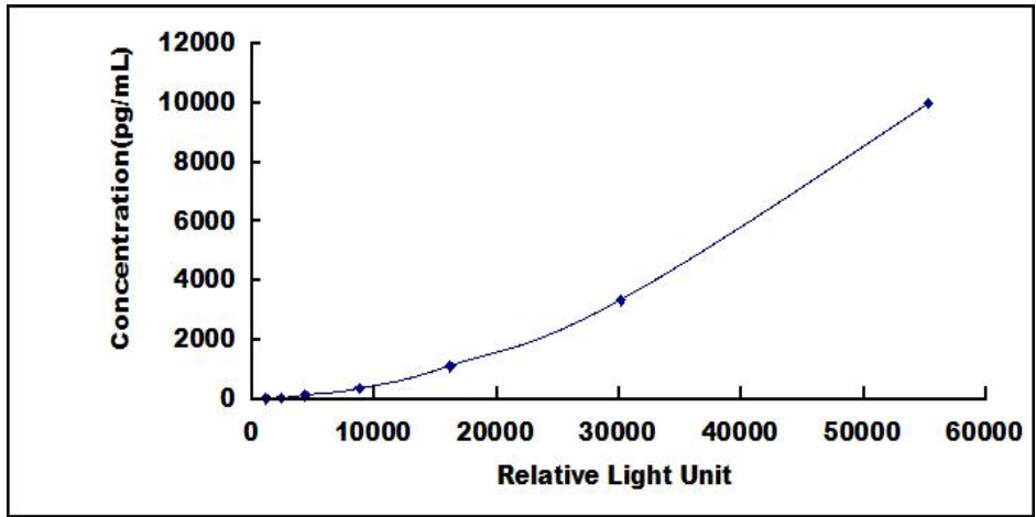
Typical Standard Curve for MUC5AC ELISA.
