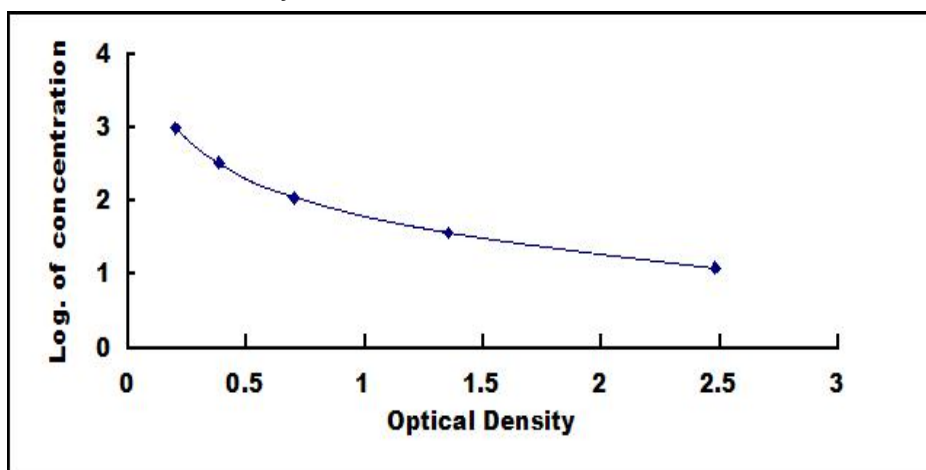
Typical Standard Curve for E2 ELISA.
