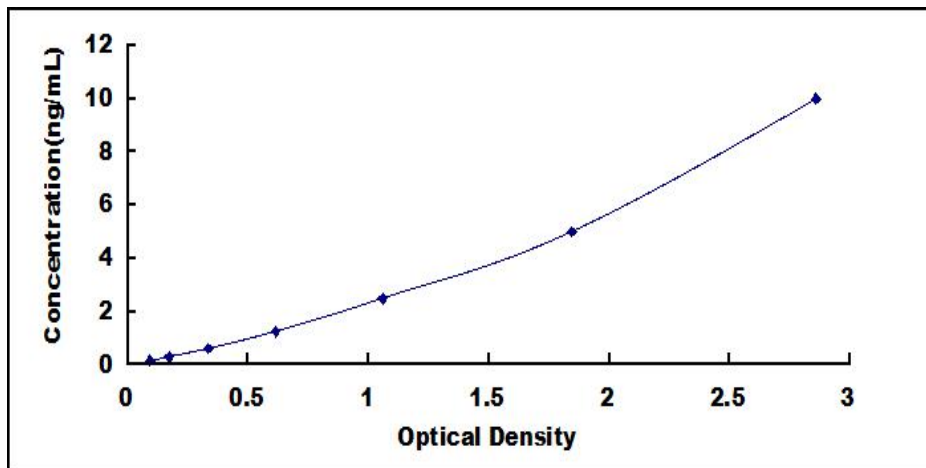
Typical Standard Curve for ANXA7 ELISA.
