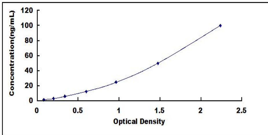
Typical Standard Curve for CLU ELISA.
