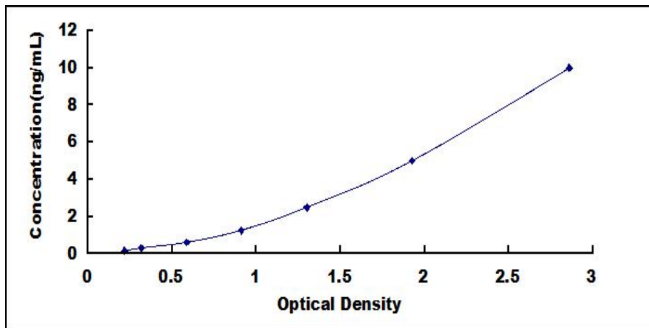
Typical Standard Curve for PYCARD ELISA.
