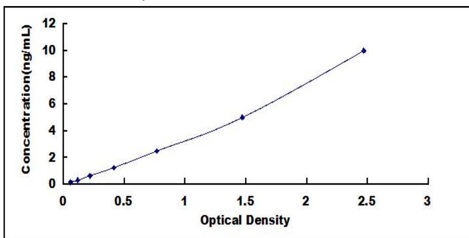
Typical Standard Curve for SOD ELISA.
