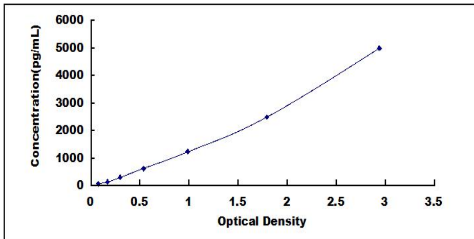
Typical Standard Curve for TACTILE ELISA.
