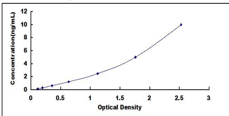
Typical Standard Curve for UCK2 ELISA.
